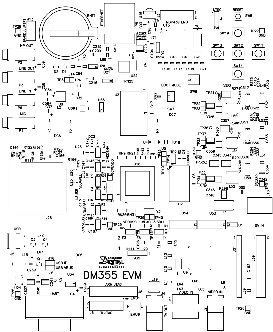
PWB 509901 REV E 10-2-08 TOP SIDE SILKSCREEN
